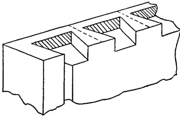
FIG. 431. CENTER LINES FOR TENONS.
